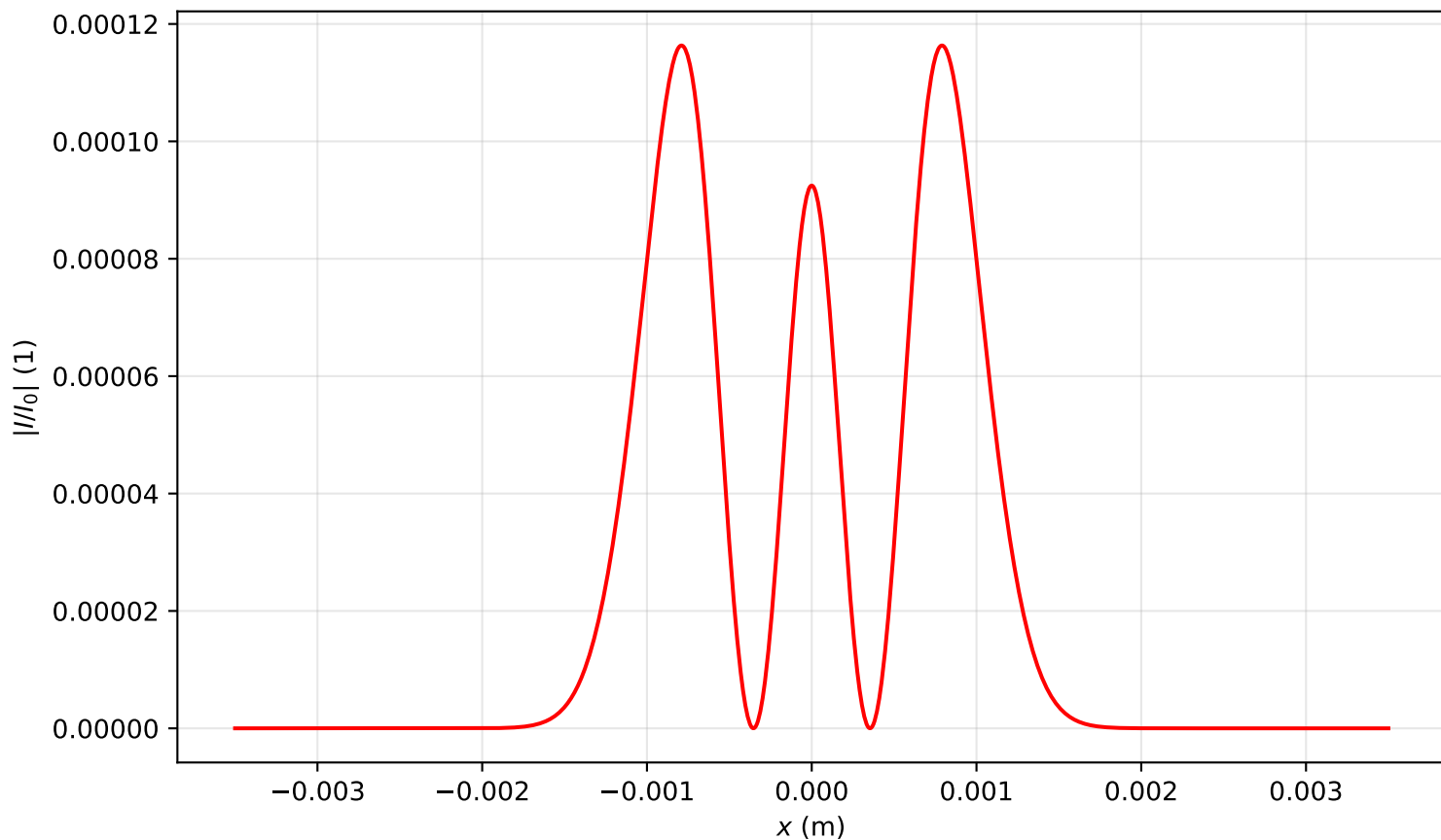
Intensity profile I(x, y = 0, z = 0.318)/I_0 , P_{in}=1.0P_{cr} , artificial time
